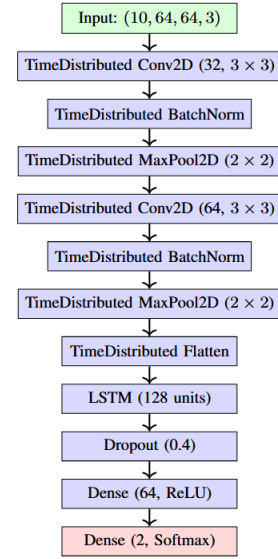
Fig. 3. Block diagram of the Tier 1 CNN–LSTM spatio-temporal network architecture.
