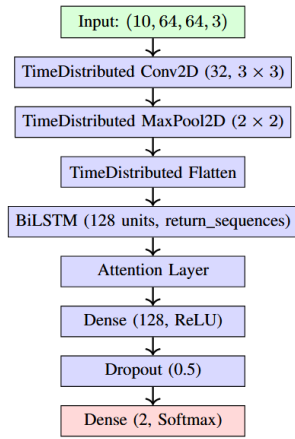
Fig. 4. Block diagram of the Tier 2 CNN-BiLSTM-Attention model architecture.
